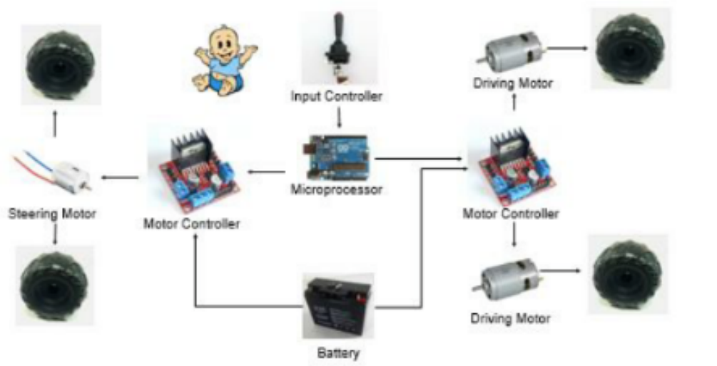
Figure 32 Schematics of The Parts
